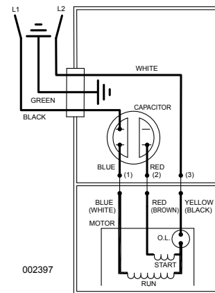
002397 WIRING DIAGRAM FOR MODELS "E295-A" thru "E295-G" 7/85 (TR) thru Current
