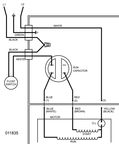
011835 WIRING DIAGRAM FOR MODELS "WD295-A" thru "WD295-D" 3/98 thru Current
