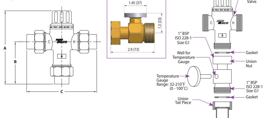
5120 Series Mixing Valve Dimensions Dimensions for reference only
