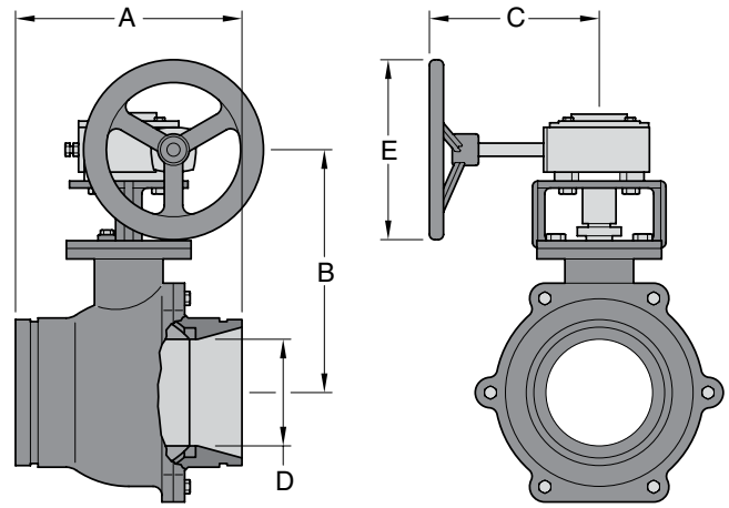
BV835 BALL VALVE WITH GEAR OPERATOR
