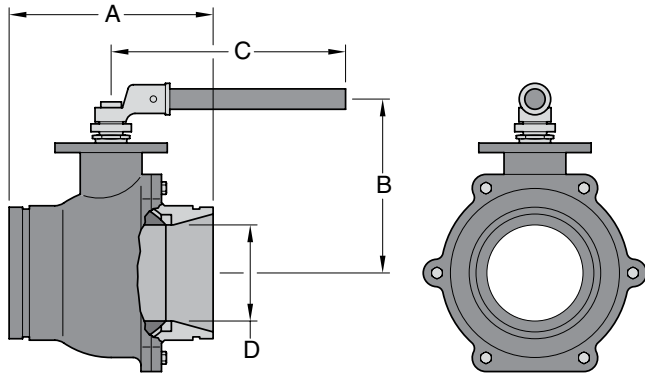
BV835 BALL VALVE WITH LEVER HANDLE
