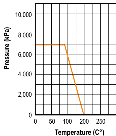
MODEL BV835 BALL VALVE PRESSURE PERFORMANCE
